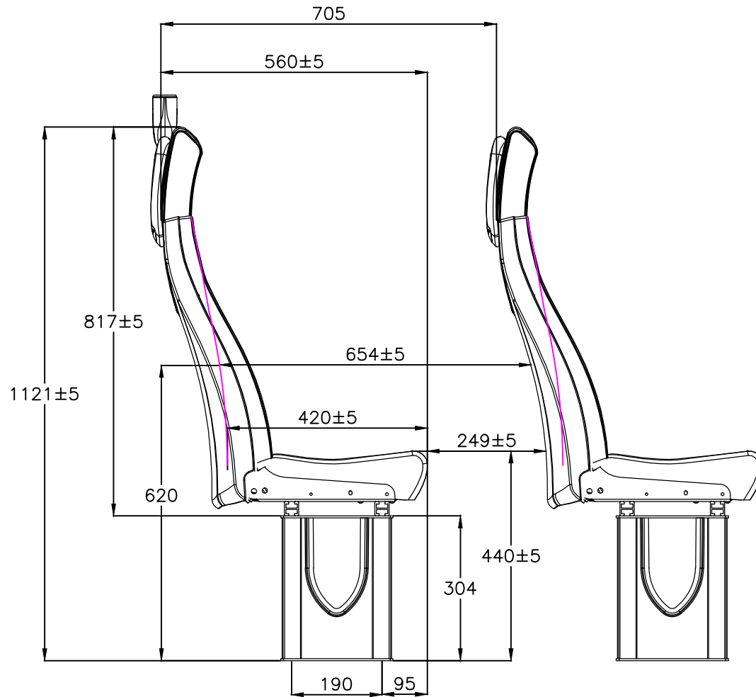
- Side view -
